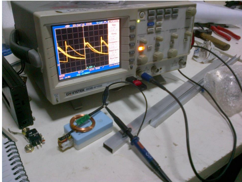
7. Pengukuran Output Receiver Tanpa Beban
