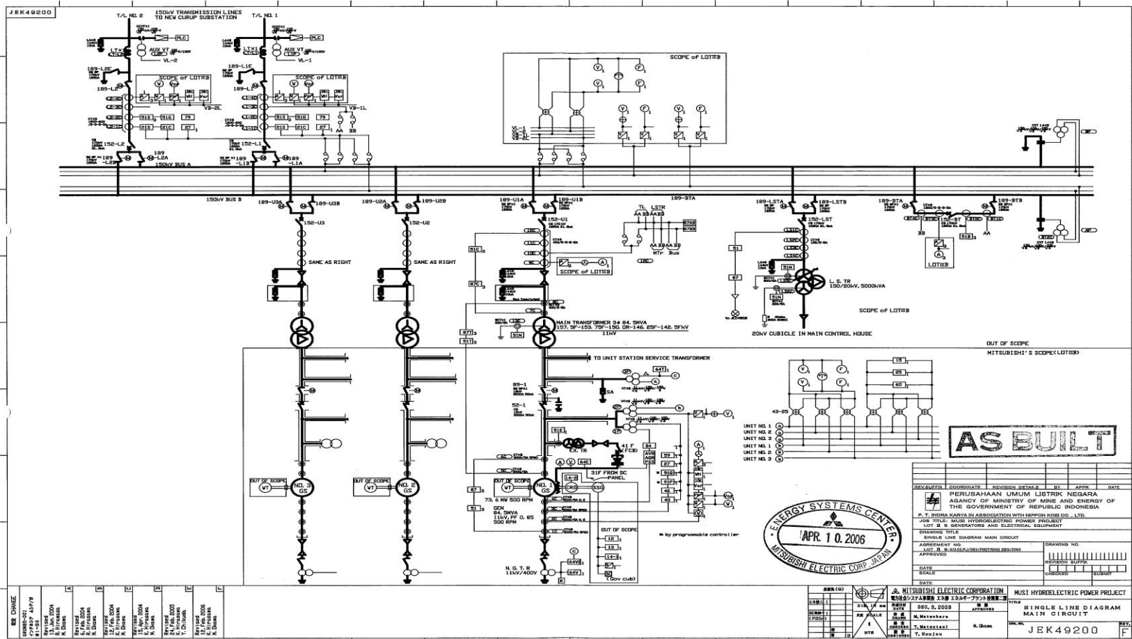
Lampiran 1 : Single Line Diagram Main Circuit PLTA Musi
