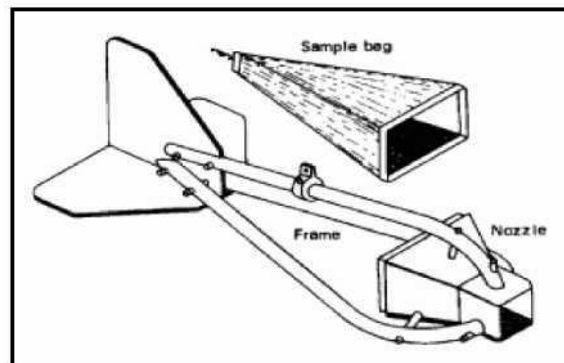
Gambar 3.5 Alat ukur sedimen dasar Helley Smith (WMO, 1989)
