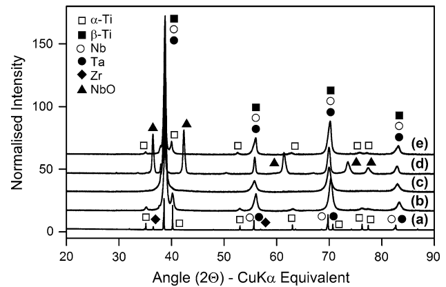
Fig. 2 Synchrotron radiation diffraction (SRD) plots of the Ti–Nb–Ta–Zr specimens: (a) mixed elemental powder, (b) after densification by hot isostatic pressing in argon (1000°C/2 h/100 MPa), (c) after densification by hot isostatic pressing in argon (1100°C/4 h/100 MPa), (d) after isothermal foaming at 1150°C/10 h, (e) after isothermal foaming at 1350°C/10 h. Note that the presence of NbO in the specimen foamed at 1150°C was attributed to reduced vacuum conditions during a portion of the treatment
