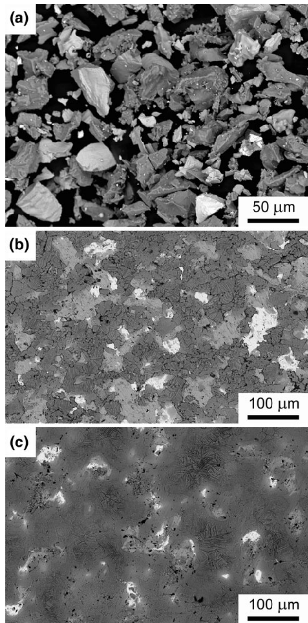
Fig. 1 Backscattered scanning electron micrographs: a illustrating the size and morphology of the blended powder, and illustrating the grain structure and degree of reaction for the Ti–Nb–Ta–Zr specimens following HIP-ing in argon: b 1000°C/2 h/100 MPa, and c 1100°C/4 h/100 MPa
