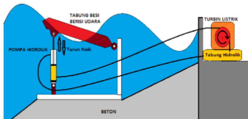
Gambar 2.8 Skema Prinsip Kerja PLTGL-OWC ( Oscillating Water Column )
