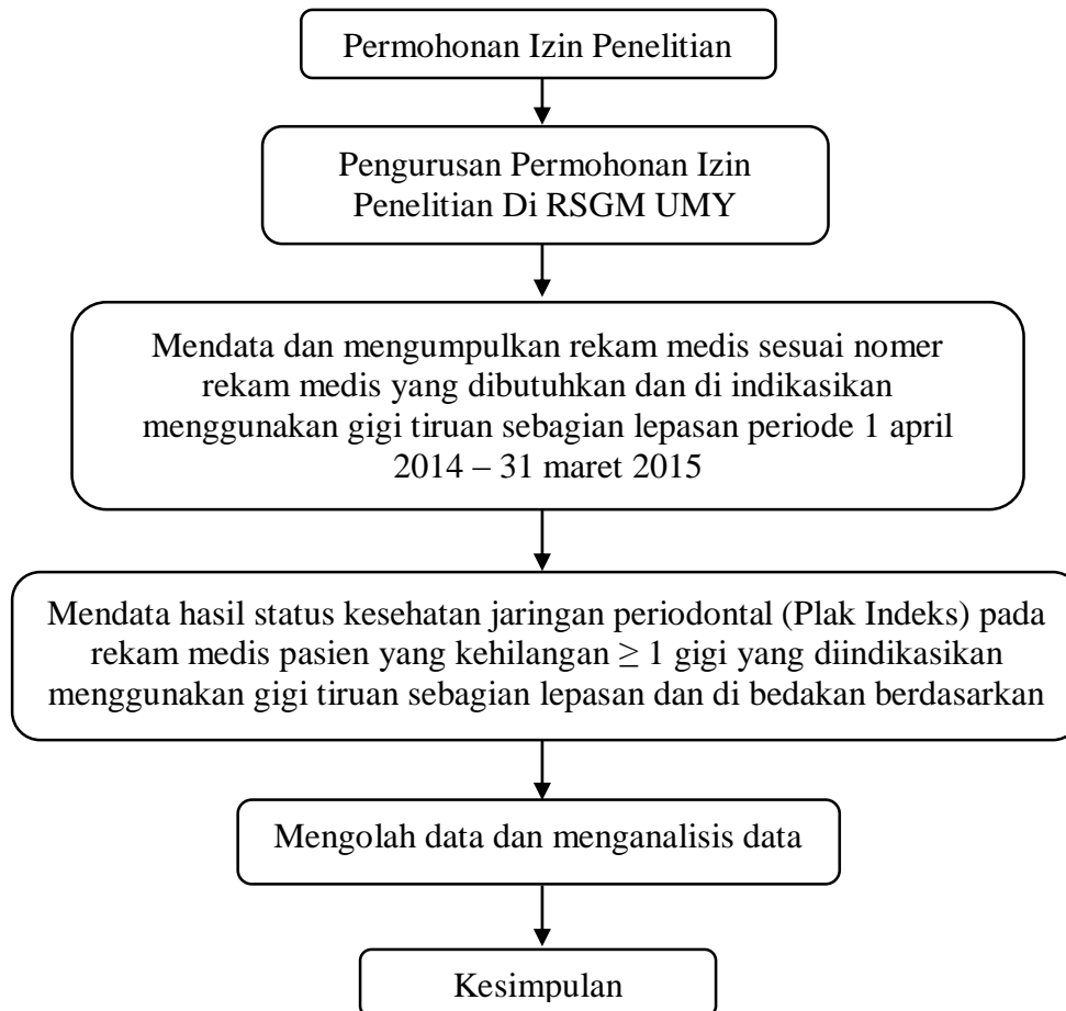
Gambar 3. Alur Penelitian
