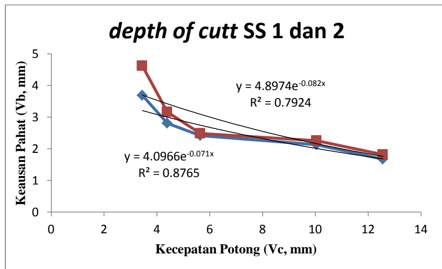
Gambar 4.18 grafik Stainless steels depth of cutt 1 dan 2.
