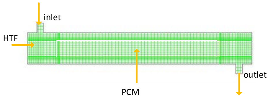
Gambar 3. Hasil meshing .
