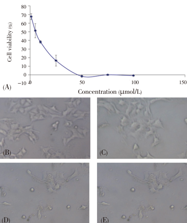
Figure 1. The effect of hesperidin on viability of MCF-7/Dox cells.
