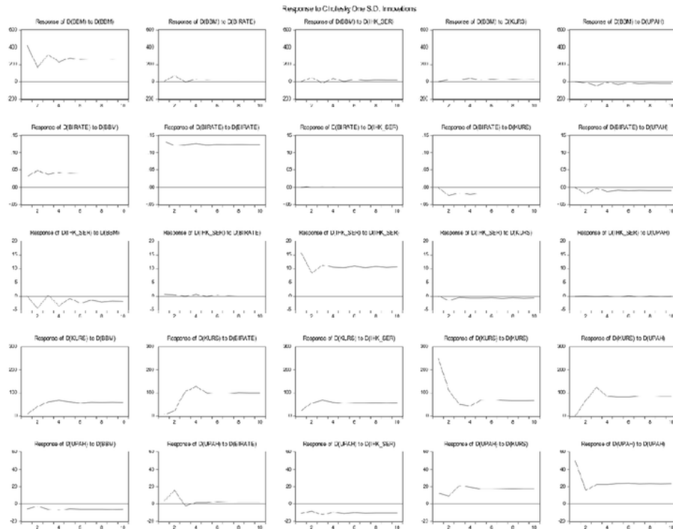
Figure 4: Impulse-Response Function (IRF)
