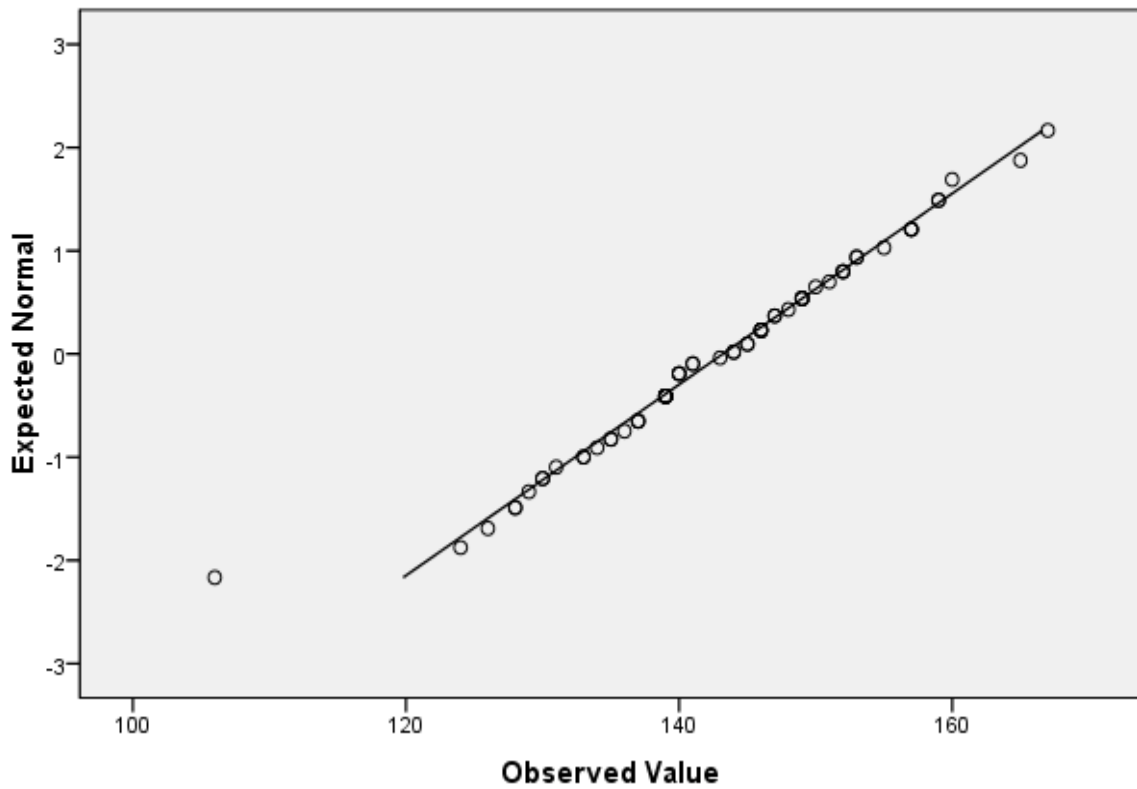
Normal Q-Q Plot of scoretotal
