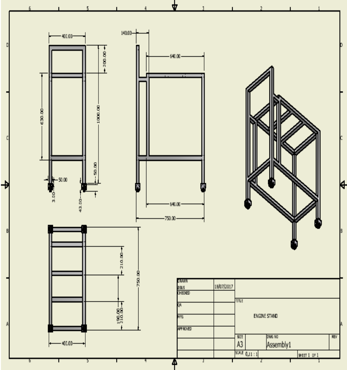
Gambar 1. Engine stand
