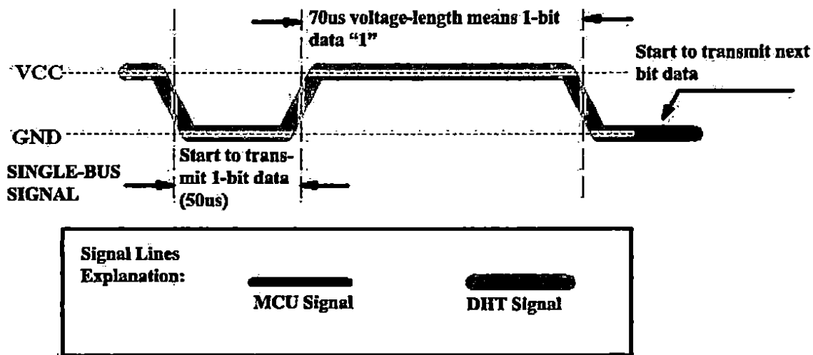
Figure 5 Data "1" Indication
