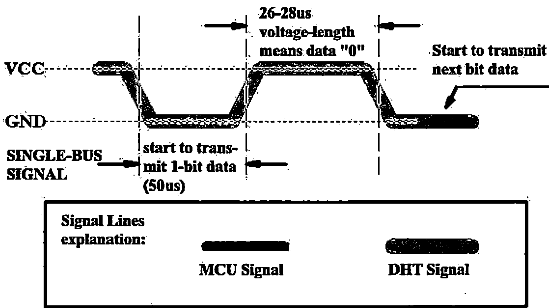
Figure 4 Data "0" Indication
