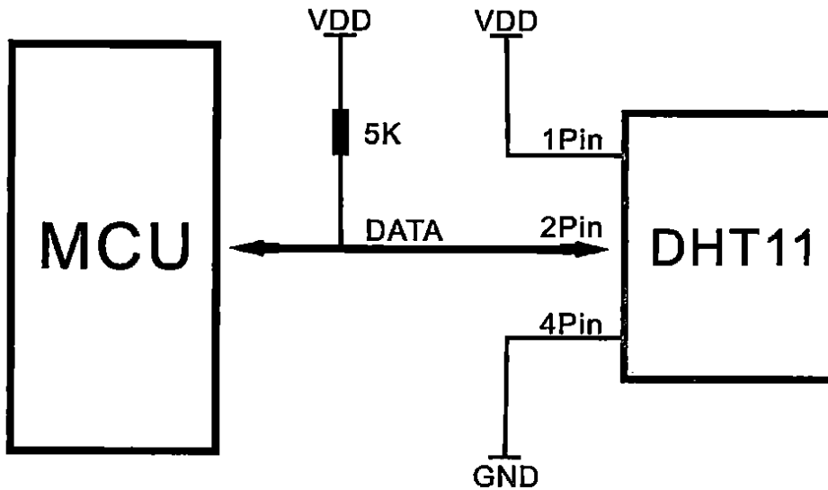
Figure 1 Typical Application
