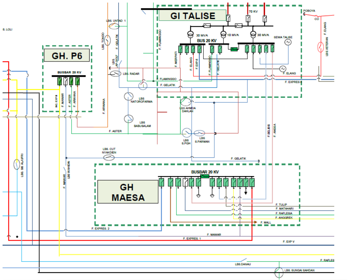
Gambar Diagram Single Line Gardu Induk Talise
