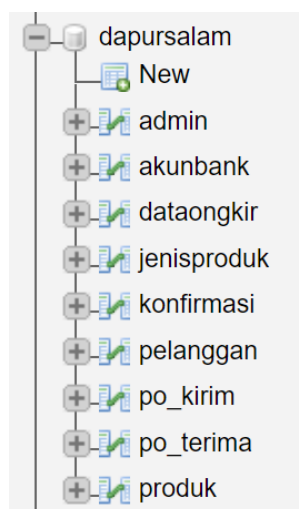
Gambar 4.1 Database DapurSalam
