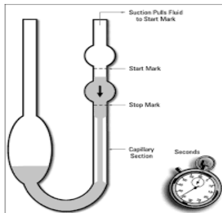
Gambar 2.14 Viskometer Oswald
