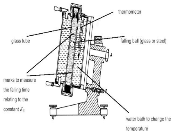
Gambar 2.15 Viskometer Hoppler
