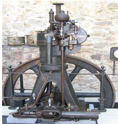
Gambar 2.1. Mesin diesel silinder tunggal Rudolf Diesel (Budiman, 2017)
