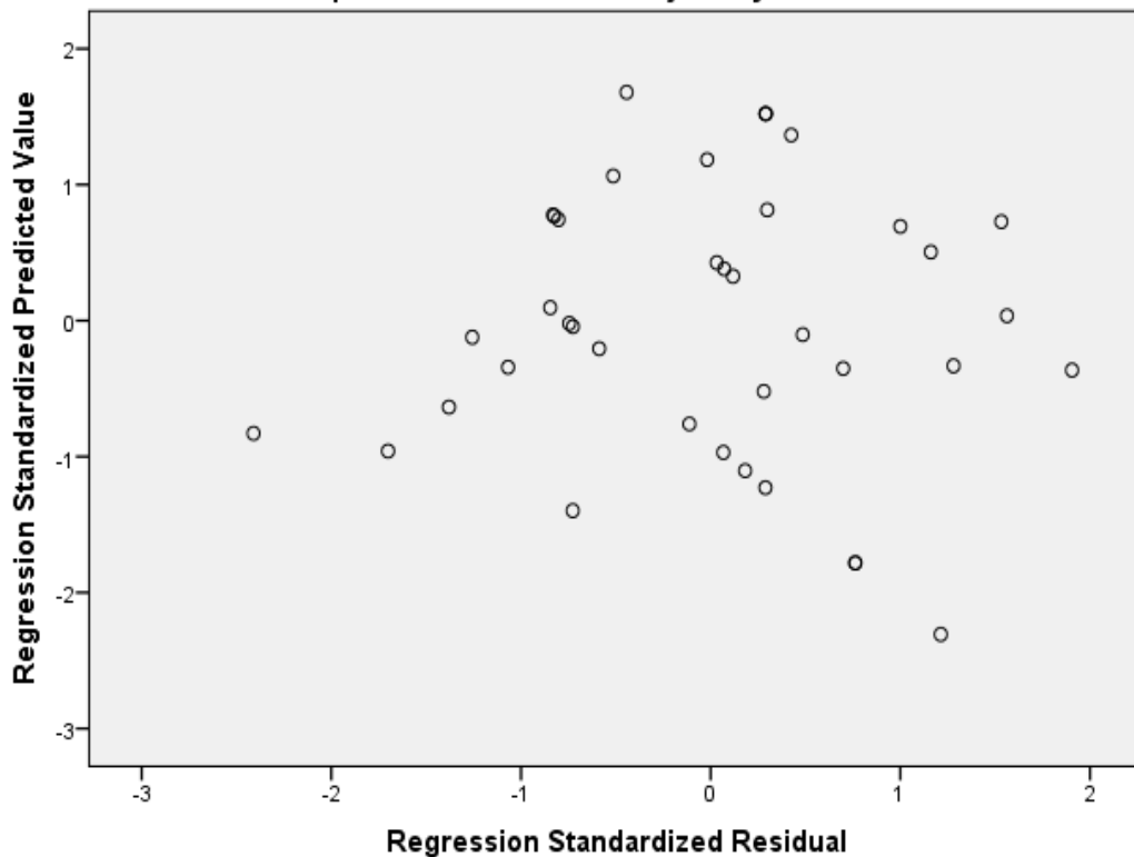
Scatterplot
