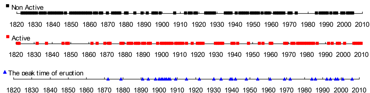
Gambar 1. Periode Keaktifan Gunung Merapi (Ikhsan, 2014)
