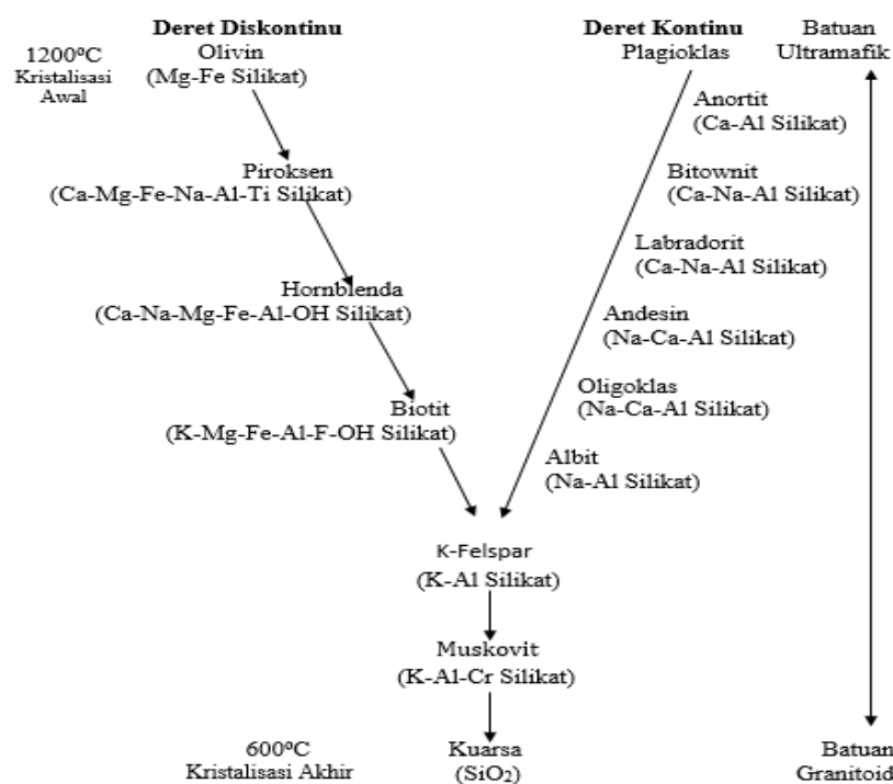
Gambar 3. Reaksi Bowen (Goldschmidt, 1958; Mason, B. & Carleton B.M., 1982)
