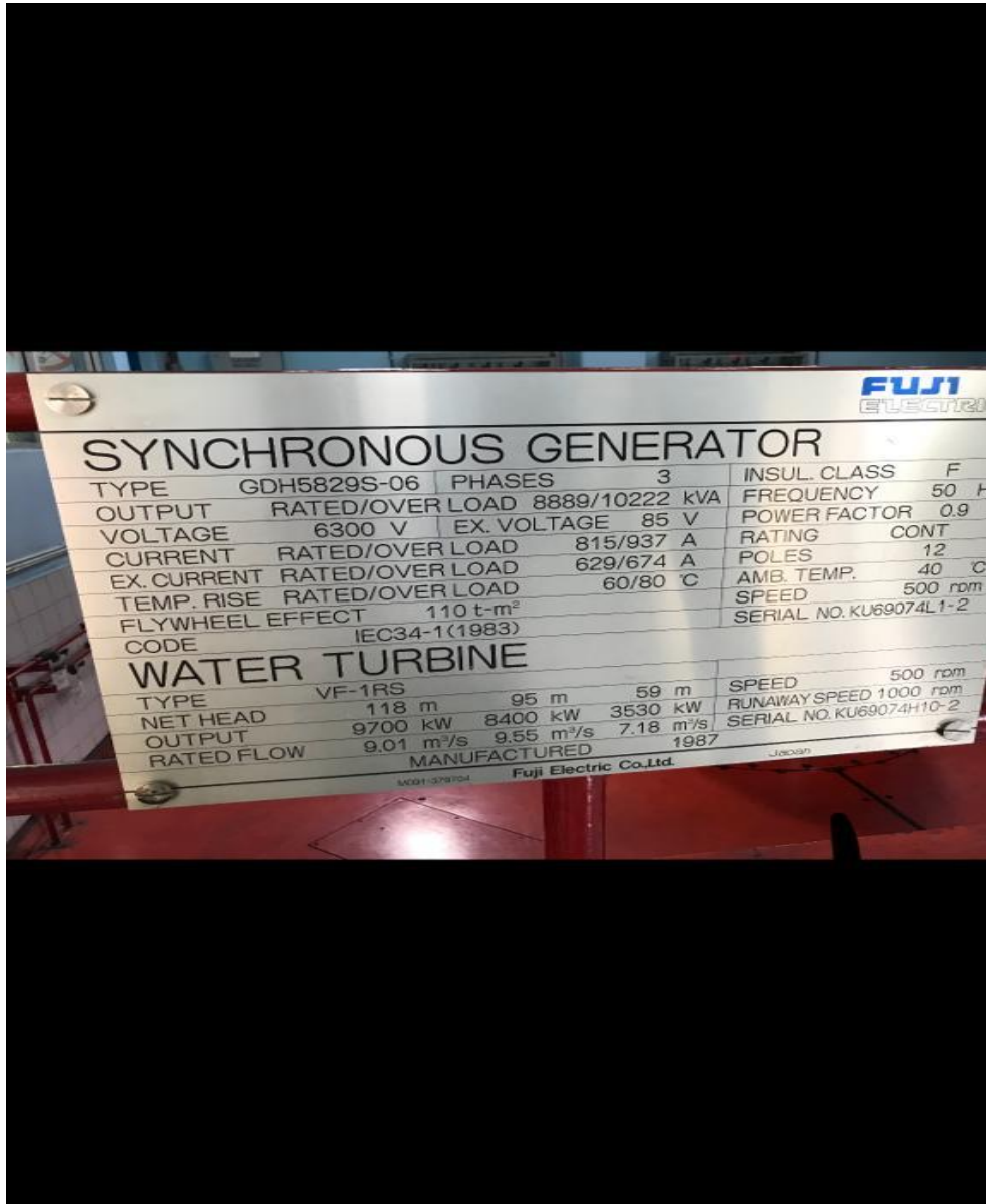
Lampiran 3. Nameplate Turbine Generator PLTA Wadaslintang
