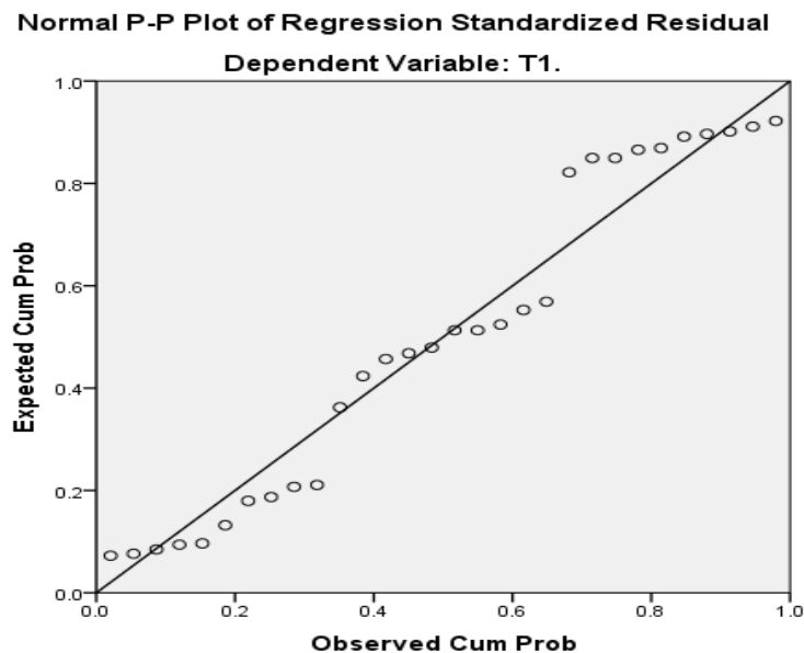
Gambar 4.1 Normal P-Plot
