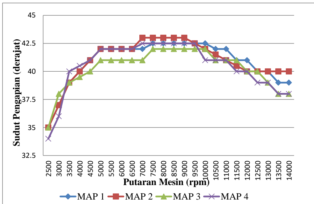
Gambar 4.3. Mapping CDI BRT I-Max + Koil standar + Busi Iridium
