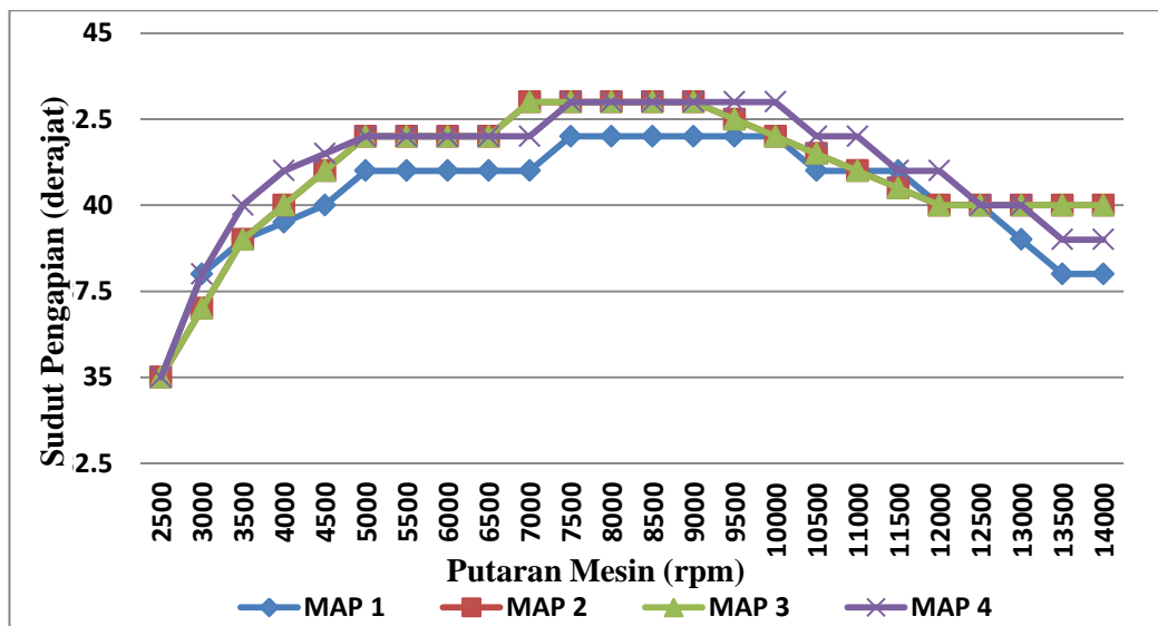
Gambar 4.6. Mapping CDI BRT I-Max + Koil TDR YZ + Busi Iridium
