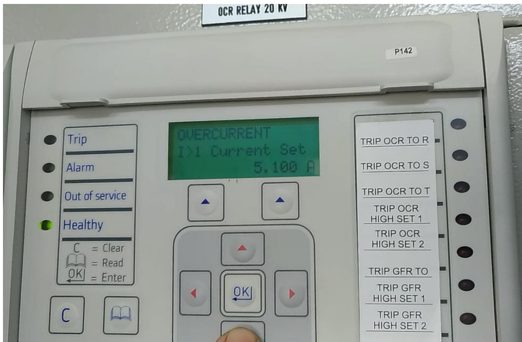
Over Current Relay 20 kV
