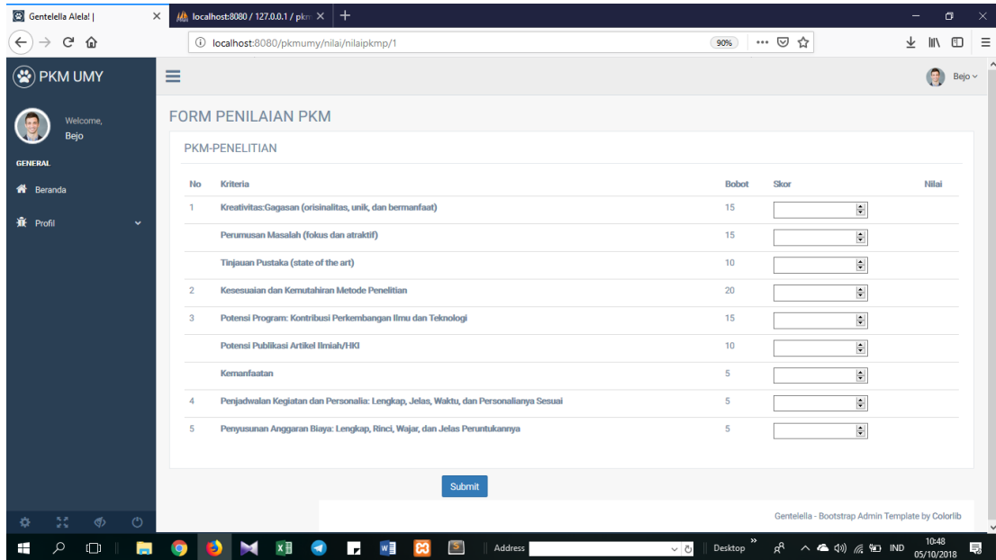
Gambar 4. 37 Halaman Penilaian
