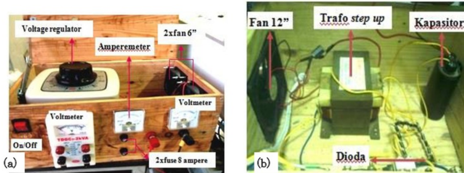
GAMBAR 7. Rangkaian power supply (a) voltage regulator (b) adaptor
