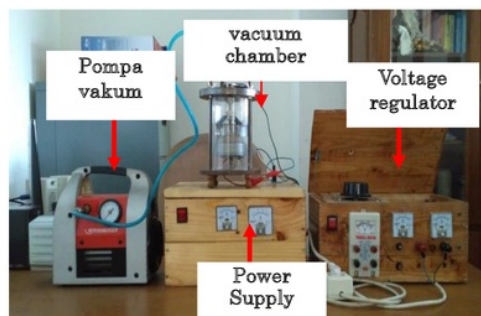
GAMBAR 9. Mesin sputtering .
