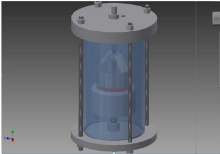
GAMBAR 4. Desain assembly vacuum chamber
