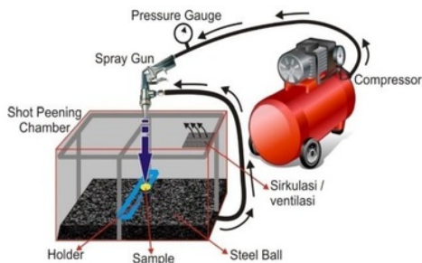
Gambar 2. Skema pengujian proses shot peening
