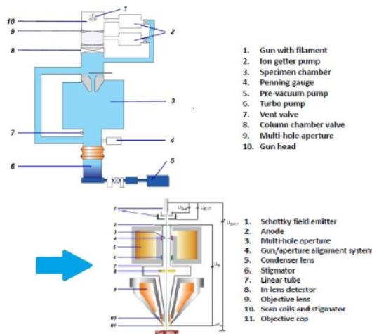
Figure 3: Principle of FE-SEM operations
