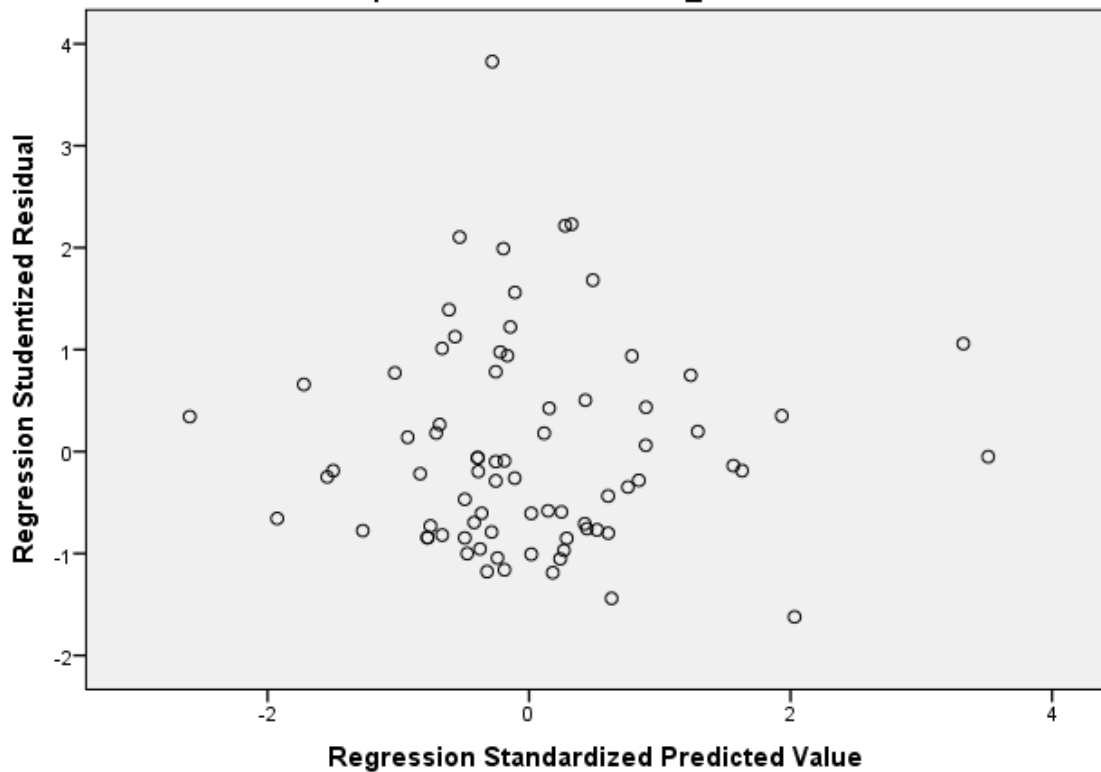
Scatterplot
