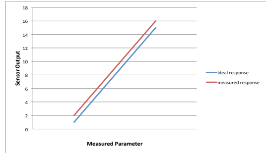
Fig. 7. One-point calibration
