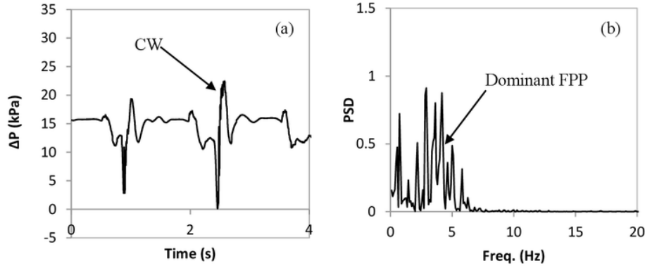
Figure 2 (a) Typical pressure difference fluctuation; (b) PSD of pressure difference, ( \dot{m}_{st}=8.4 \times 10^{-3} kg/s to \dot{m}_{st}=8.6 \times 10^{-3} kg/s), \dot{m}_{co}=5.78 \times 10^{-1} kg/s)
