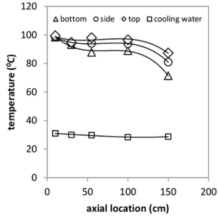
Figure 4 Temperature profile on the cross-section pipe test ( \dot{m}_{st}=6.5 \times 10^{-3} \text{ kg/s} , \dot{m}_{co}=4.23 \times 10^{-1} \text{ kg/s} )
