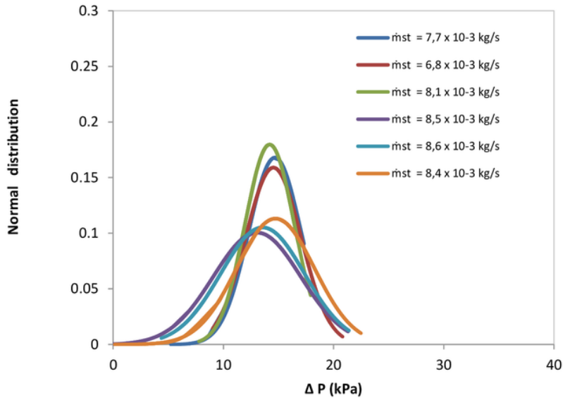
Figure 5 Normal distribution of pressure difference fluctuation ( \dot{m}_{co}= 5.78 \times 10^{-1} \text{ kg/s} )
