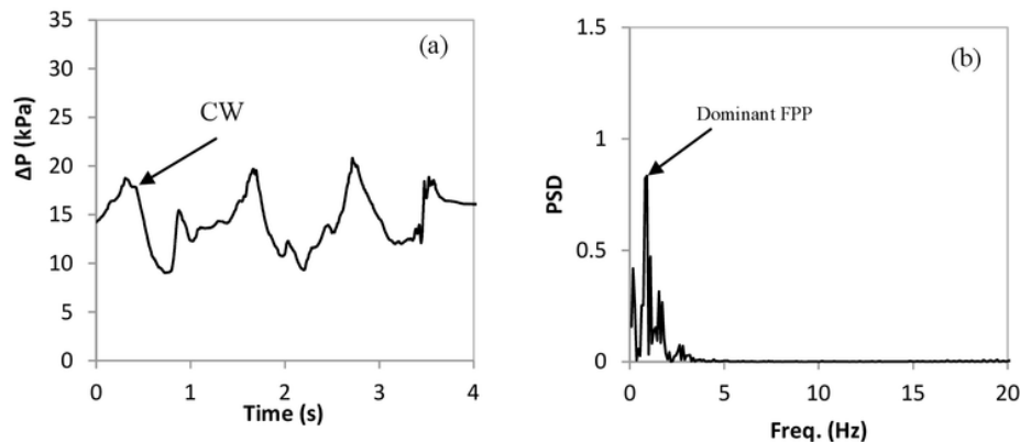
Figure 1 (a) Typical pressure difference fluctuation; (b) PSD of pressure difference, ( \dot{m}_{st} = 6.8 \times 10^{-3} kg/s to \dot{m}_{st} = 8.1 \times 10^{-3} kg/s, \dot{m}_{co} = 5.78 \times 10^{-1} kg/s)
