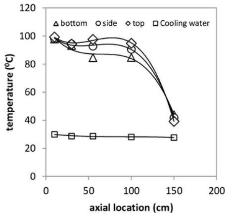
Figure 3 Typical temperature profiles on the cross-section pipe test ( \dot{m}_{st}= 2.6 \text{ kg/s} , 3.5 \times 10^{-3} \text{ kg/s} , 4.3 \times 10^{-3} \text{ kg/s} , 5.1 \times 10^{-3} \text{ kg/s} , and \dot{m}_{co}= 4.23 \times 10^{-1} \text{ kg/s} )
