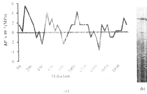
Fig.4. a) The relation of \Delta P (MPa) with time (millisecond) ( J_L ) 5 \times 10^{-3} m/s dan ( J_G ) 5 \times 10^{-3} m/s. b) Visualization of the little bubble flow pattern and slug flow pattern.
