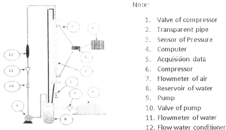
Fig. 1. Scheme of research installation
