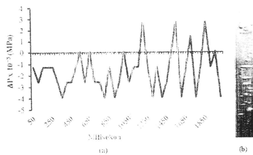
Fig. 5. a) The correlation between \Delta P (MPa) with time (millisecond) ( J_L ) 6,67 \times 10^{-3} m/s dan ( J_G ) 3,33 \times 10^{-3} m/s. b) Bubbles flow pattern visualization, big bubble.
