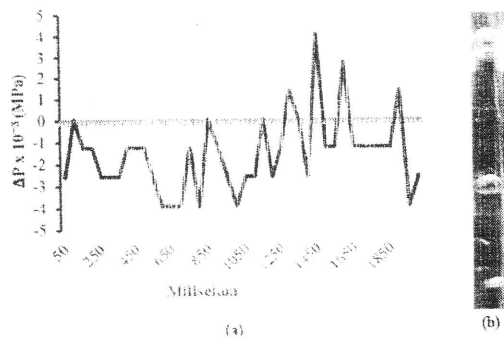
Fig. 6. a) The correlation between \Delta P (MPa) with time (millisecond) ( J_L ) 8,33 \times 10^{-3} m/s dan ( J_G ) 1,67 \times 10^{-3} m/s. b) Bubble flow pattern visualization.
