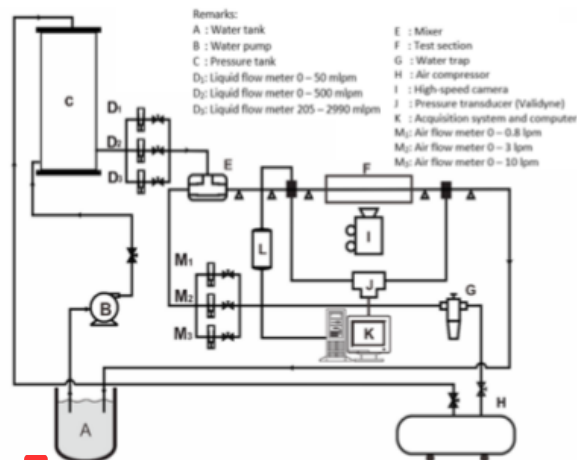
1 Figure 1. Schematic diagram of experimental apparatus
