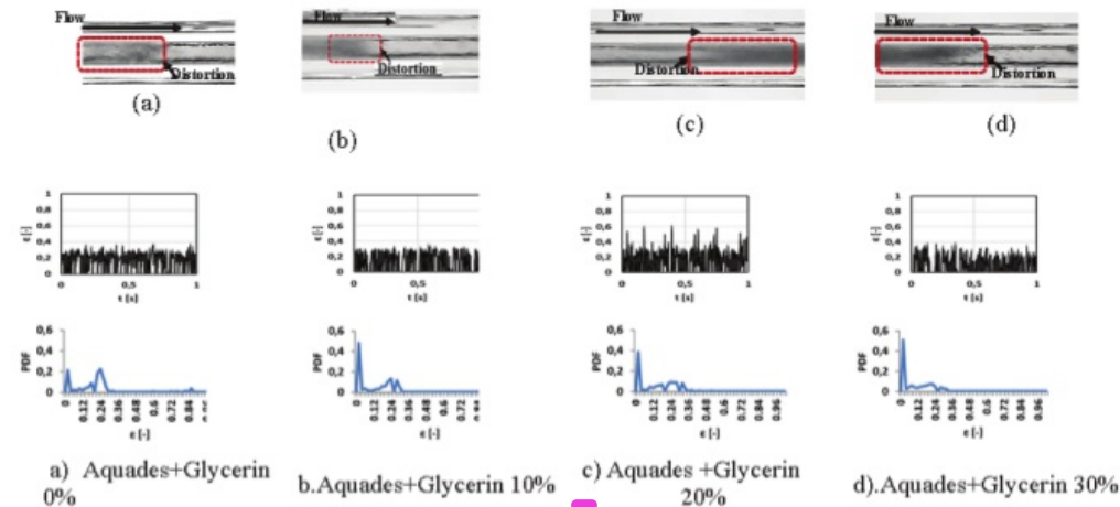
Figure 6. Churn flow pattern with J_G = 0.025 \text{ m/s} and J_L = 2.297 \text{ m/s}
