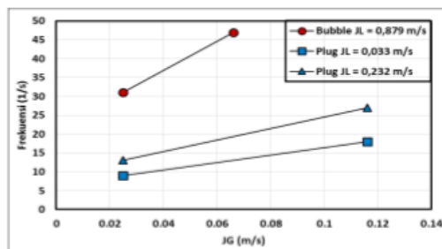
Figure 11. The Frequency of bubbly and plug
