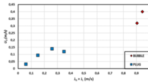
Figure 9. bubbly and plug velocity
