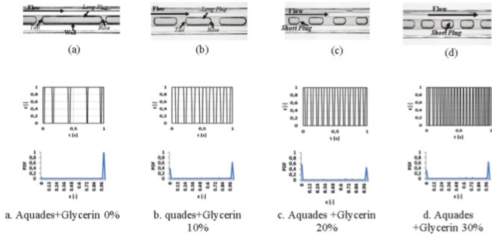
Figure 3. Plug flow pattern with J_G = 0.025 m/s and J_L = 0.033 m/s
