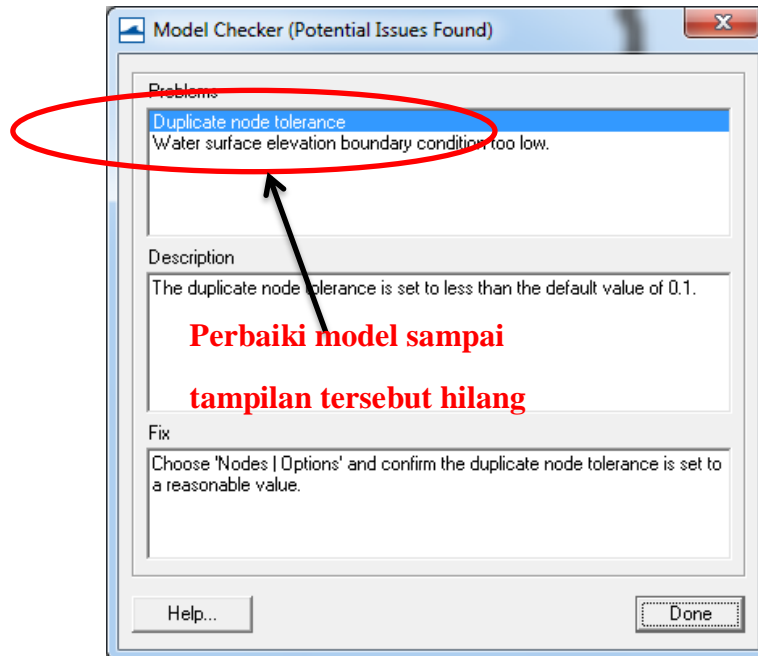
Gambar 3.57 Model Checker
