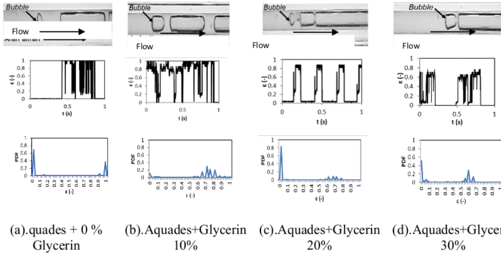
Fig. 2. Bubbly flow pattern with J_G = 0.116 m/s and J_L = 0.89 m/s
