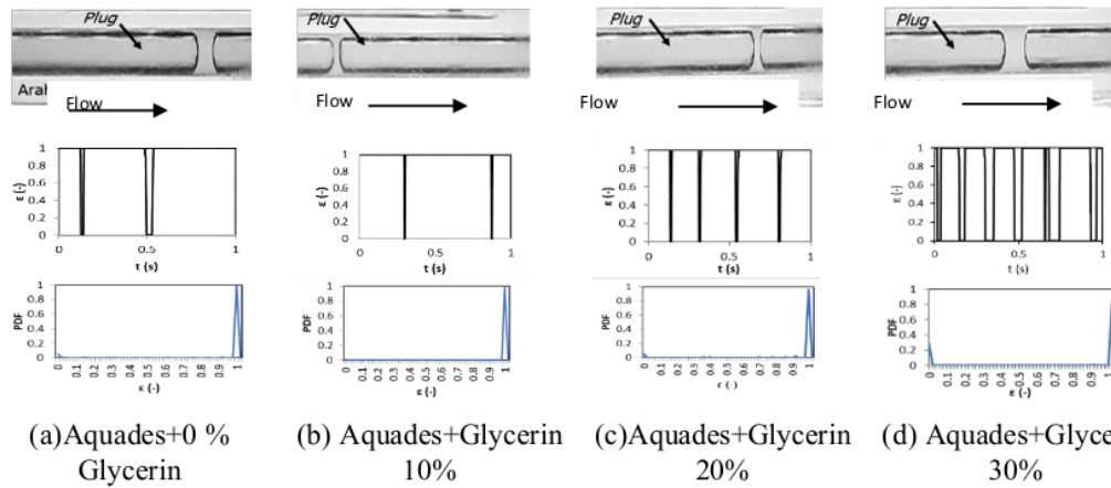
Fig. 3. Plug Flow Pattern with J_G = 0.116 m/s and J_L = 0.033 m/s
