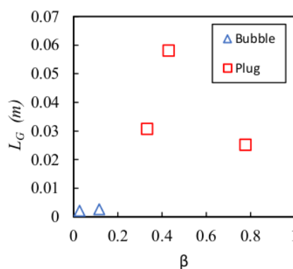
Fig. 6. The Length of Bubbly and Plug
