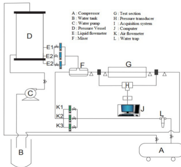
Fig. 1. Experiment set up
