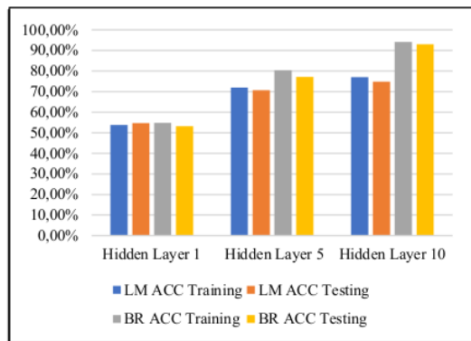
Fig. 5. Comparison of Classification Accuracy
