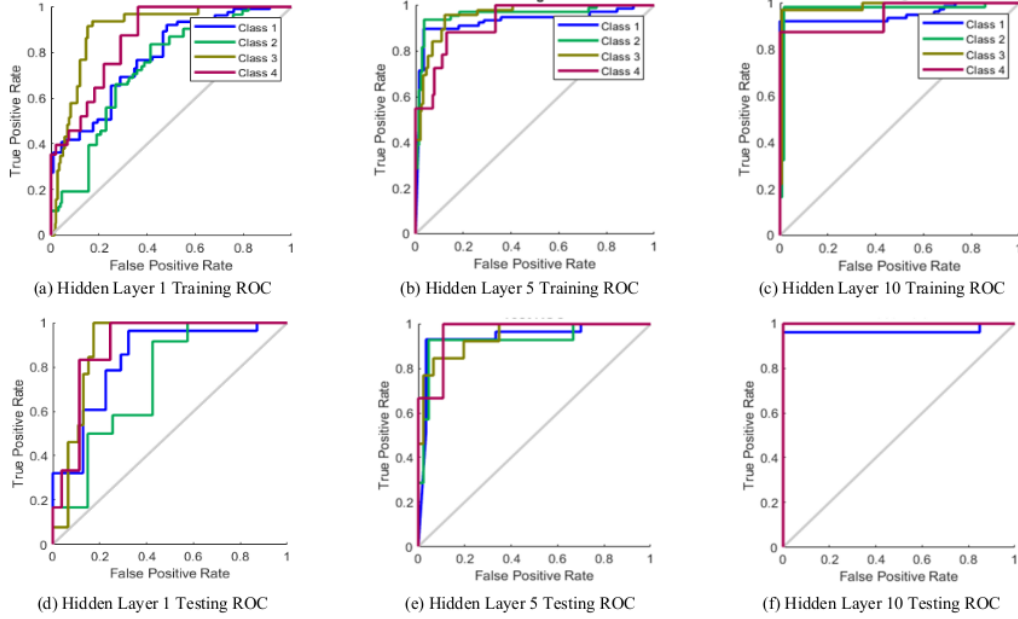
Fig. 4. ROC with Model Bayesian Regularization
