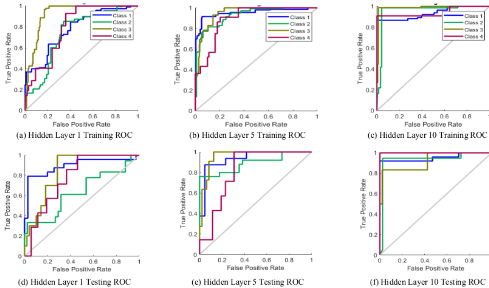
Fig. 3. ROC with Model Levenberg-Marquardt
