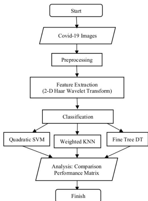
Fig. 1. System Design Flowchart.
