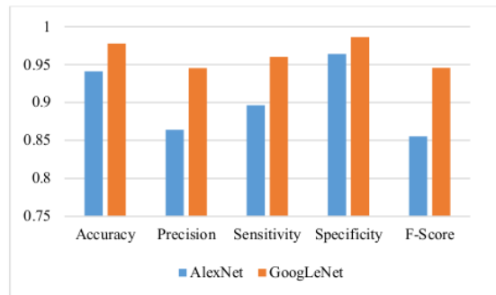
Fig. 2. Graph comparison of testing performance metrics
