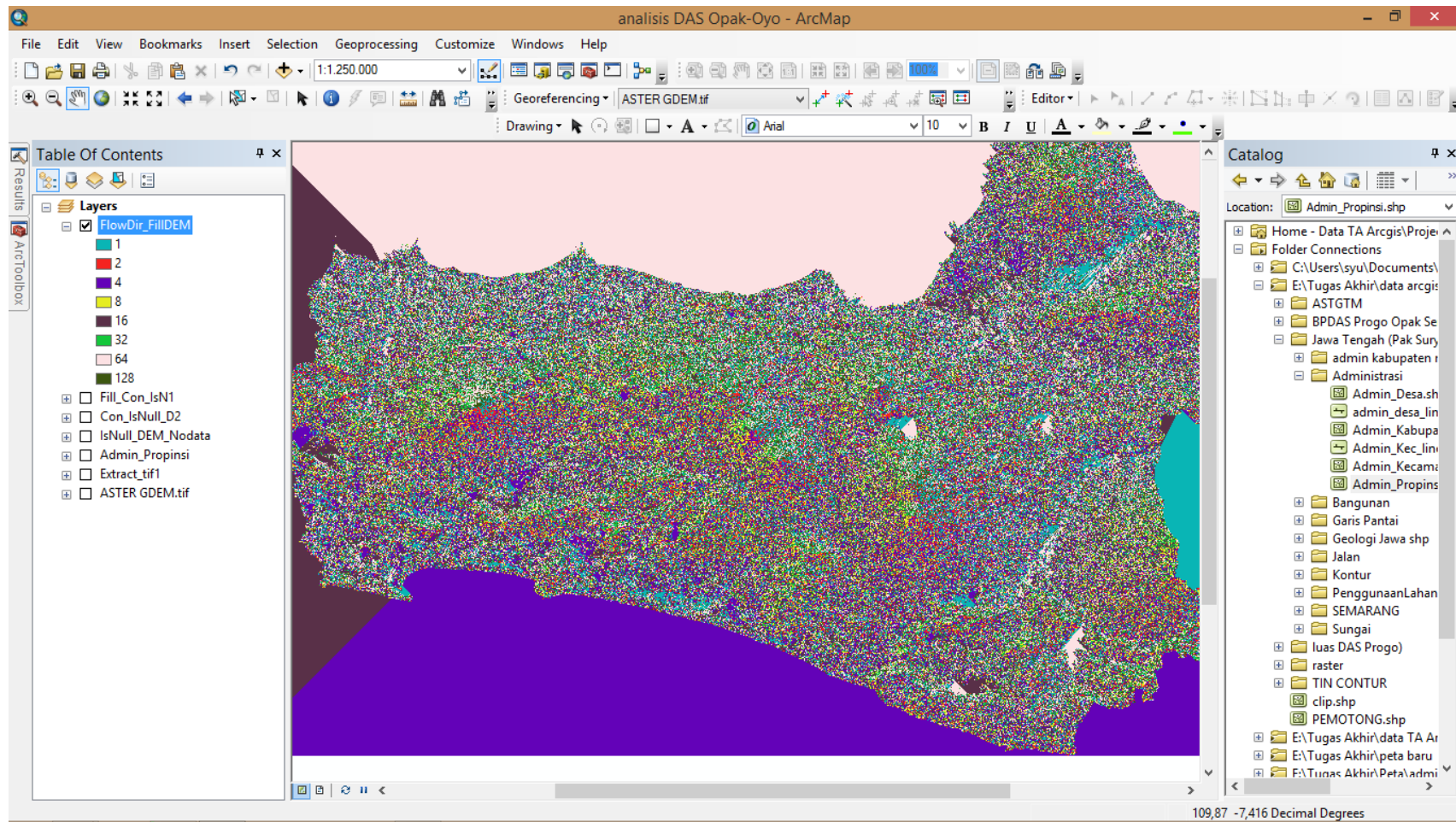
Gambar 10. Hasil Flow Direction
