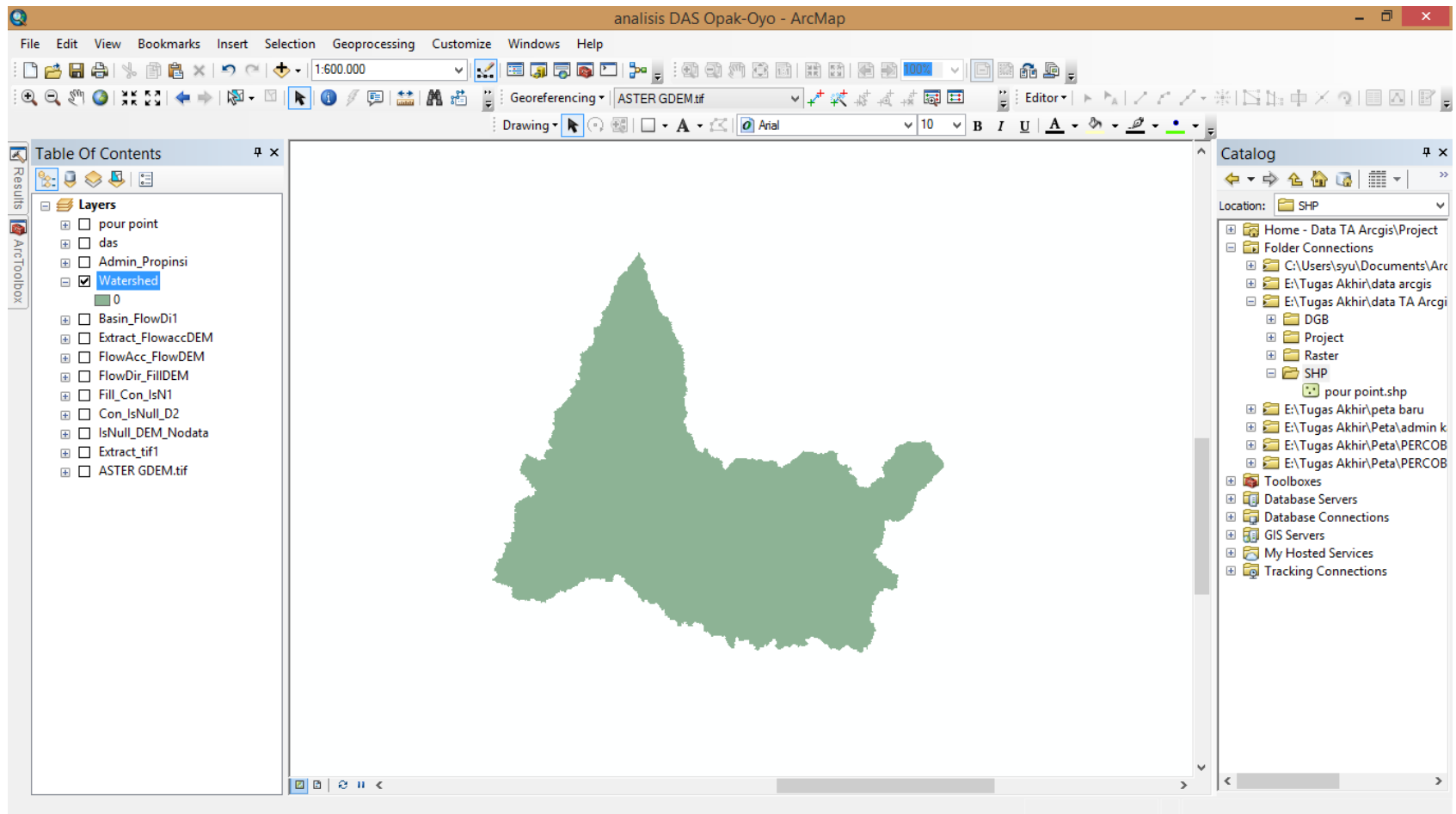
Gambar 13. Hasil Proses Watersheed
