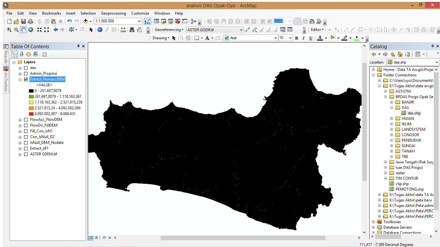
Gambar 11. Hasil Flow Accumulation
