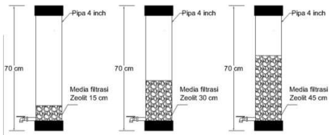
Gambar 4.4 Alat Uji Model Filtrasi Media Filtrasi Zeolit.
