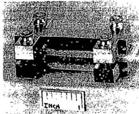
FIG. 3 Support Jig for Thin Specimen
