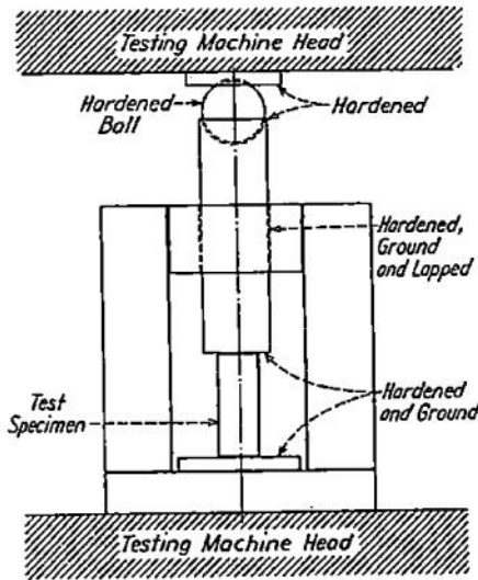
FIG. 2 Compression Tool
