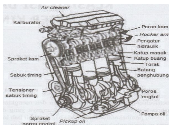
Gambar 2.1 Motor Bakar Torak (Kristanto, 2015)
