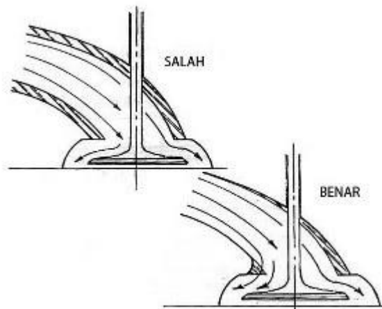
Gambar 3.8. Porting
