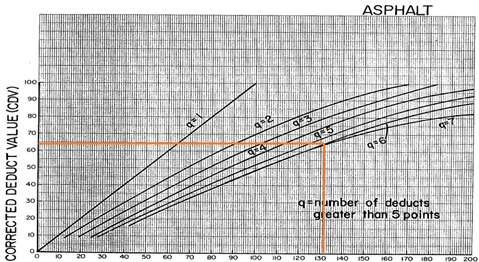
Gambar 2. Grafik CDV STA 5+100 S/D 5+200
