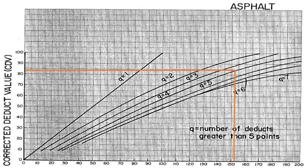
Gambar 9. Grafik CDV STA 5+800 S/D 5+900
