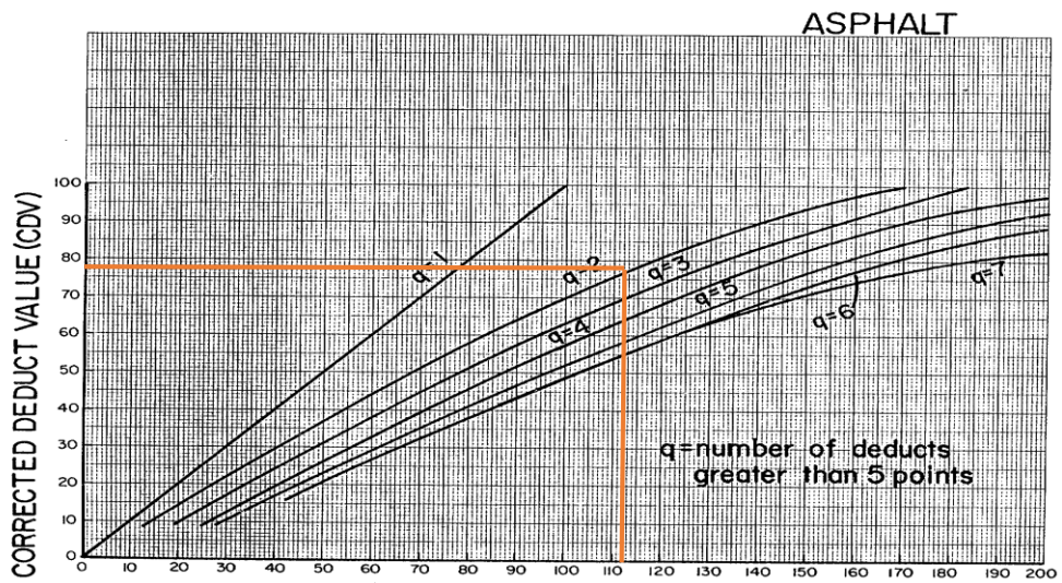
Gambar 8. Grafik CDV STA 5+700 S/D 5+800
