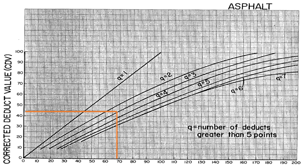
Gambar 3. Grafik CDV STA 5+200 S/D 5+300
