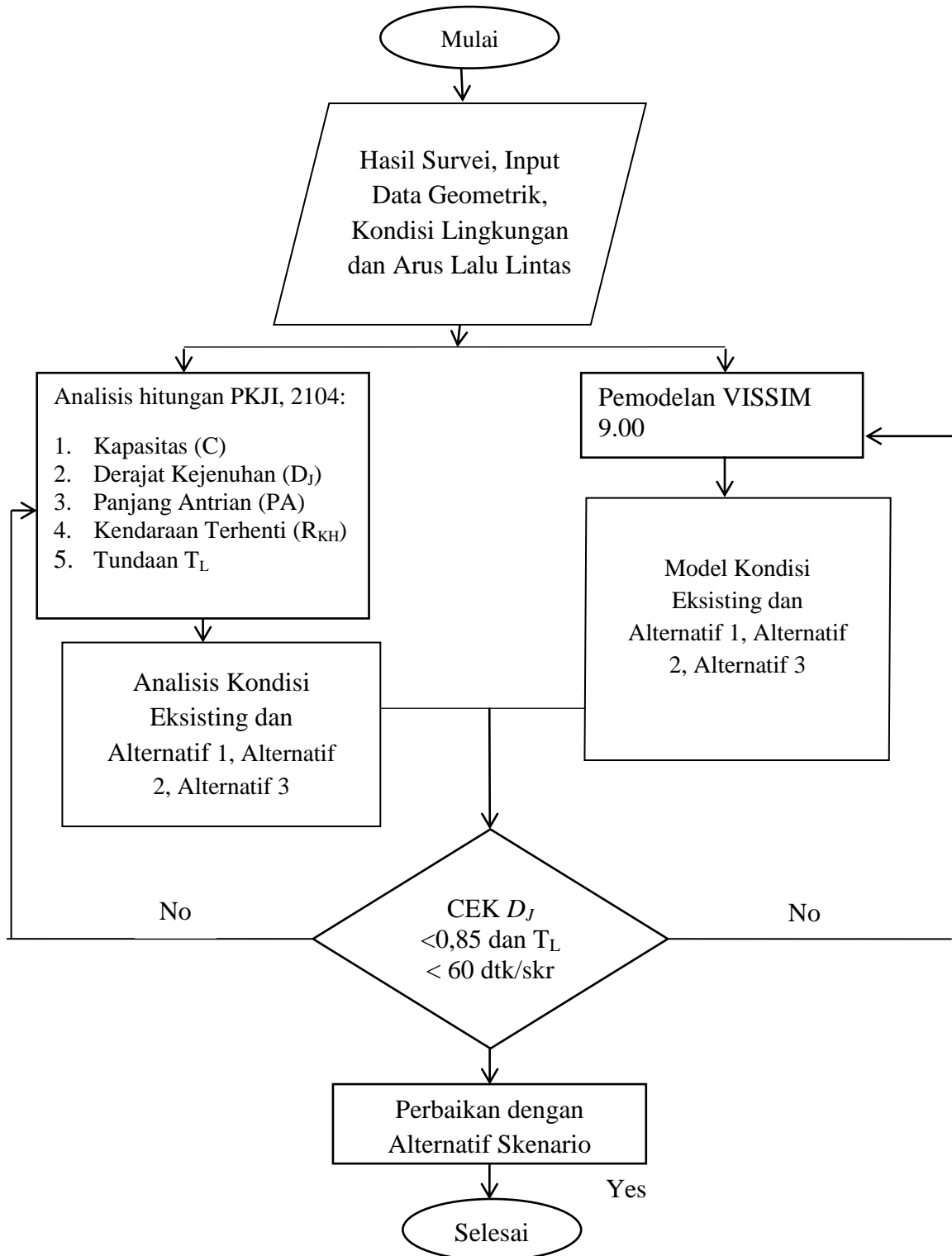
Gambar 4.3 Diagram Alir Proses Analisa Data
