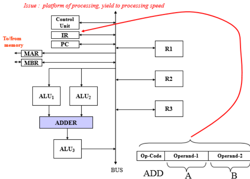
Gambar 6.1 Processor Organization
