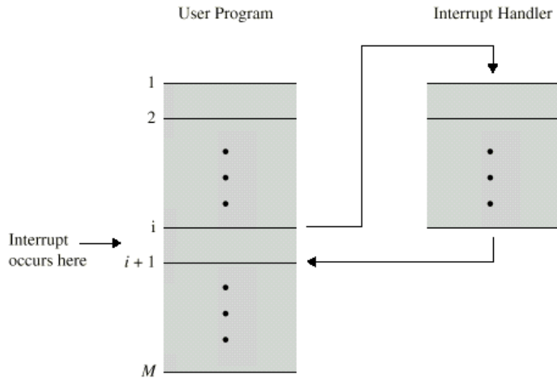
Gambar 5.1 Proses Interupsi transfer of command
