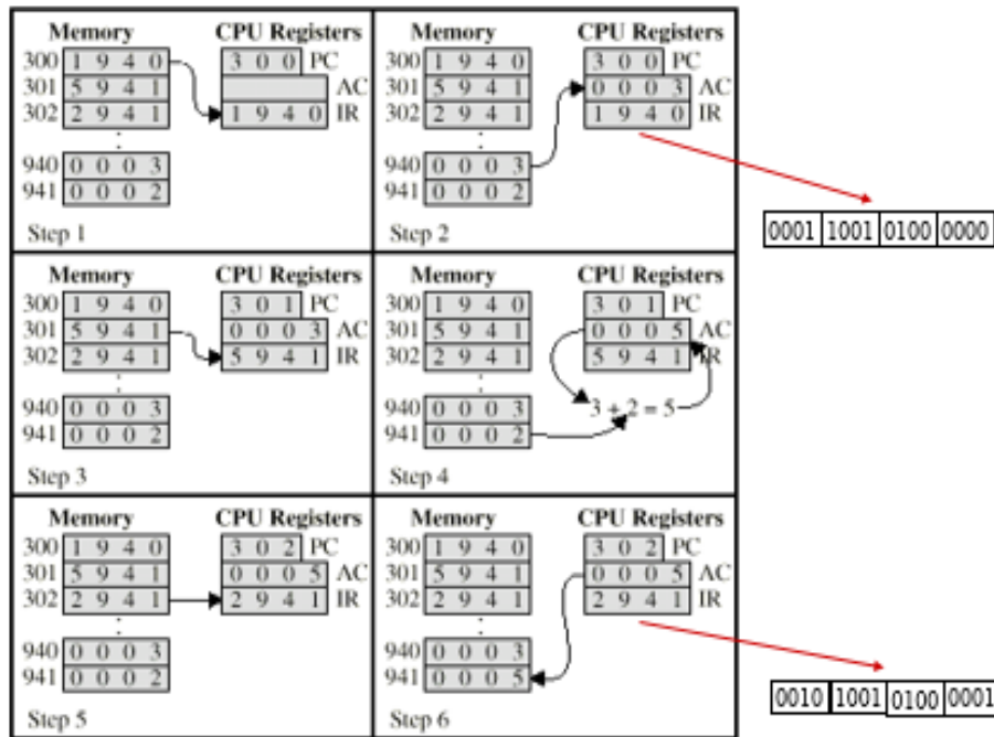
Gambar 4. 8 Contoh execution in hypothetical machine
