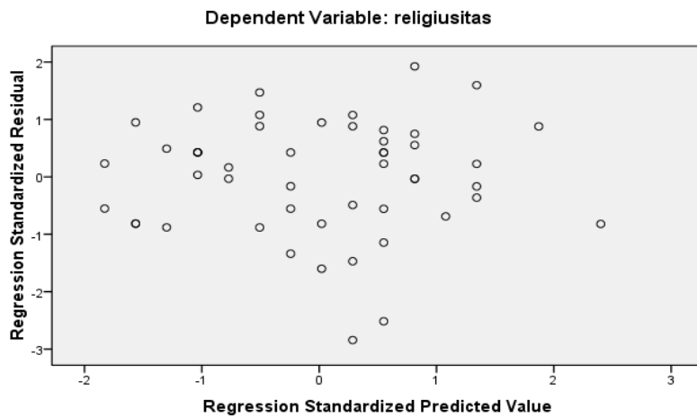
Scatterplot
