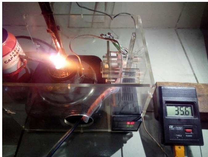
Gambar 3.19 Flash point tester
