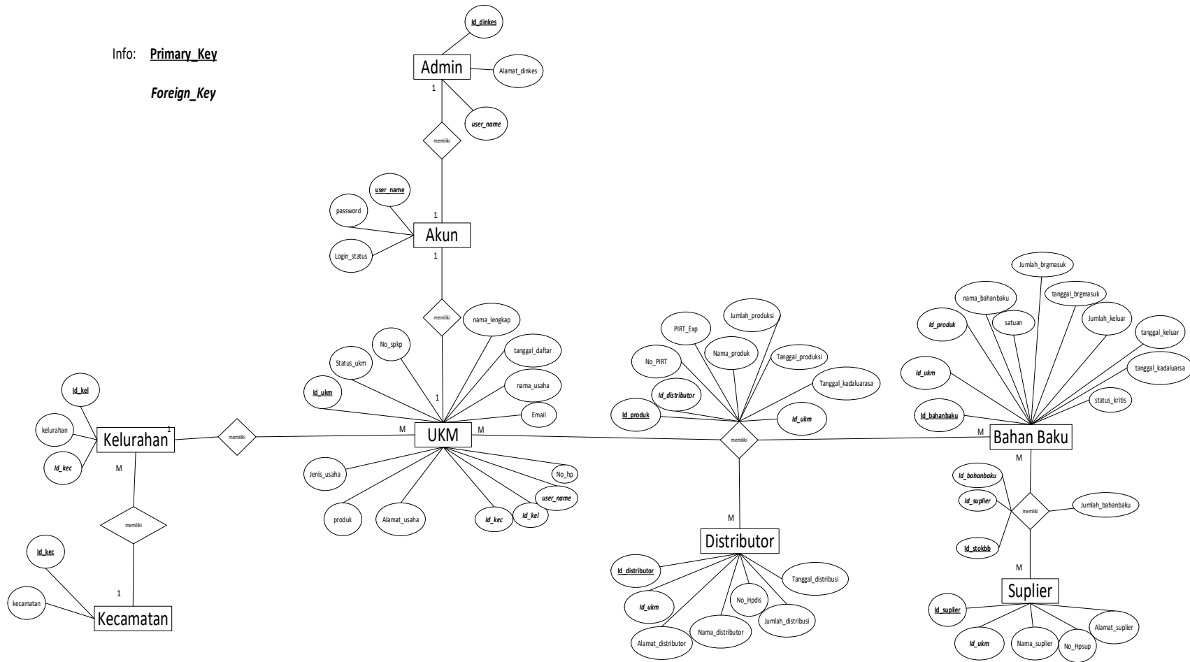
Gambar 4.4 Entity Relationship Diagram
