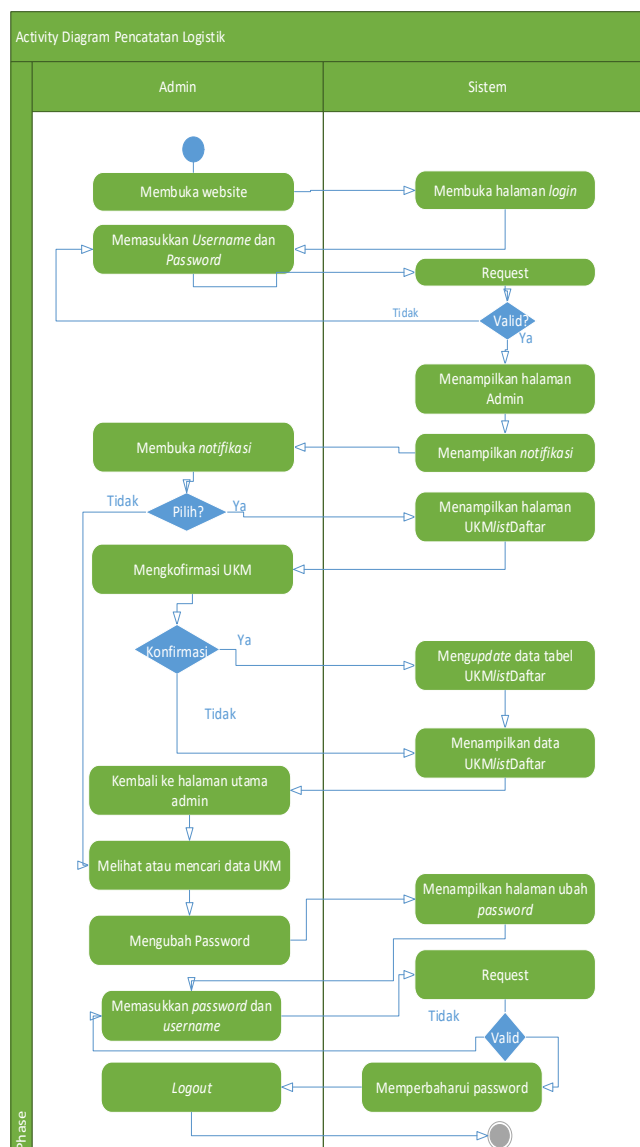
Gambar 4.2 Activity Diagram (Admin)
