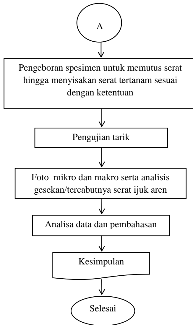
Gambar 3.32 Diagram alir penelitian
