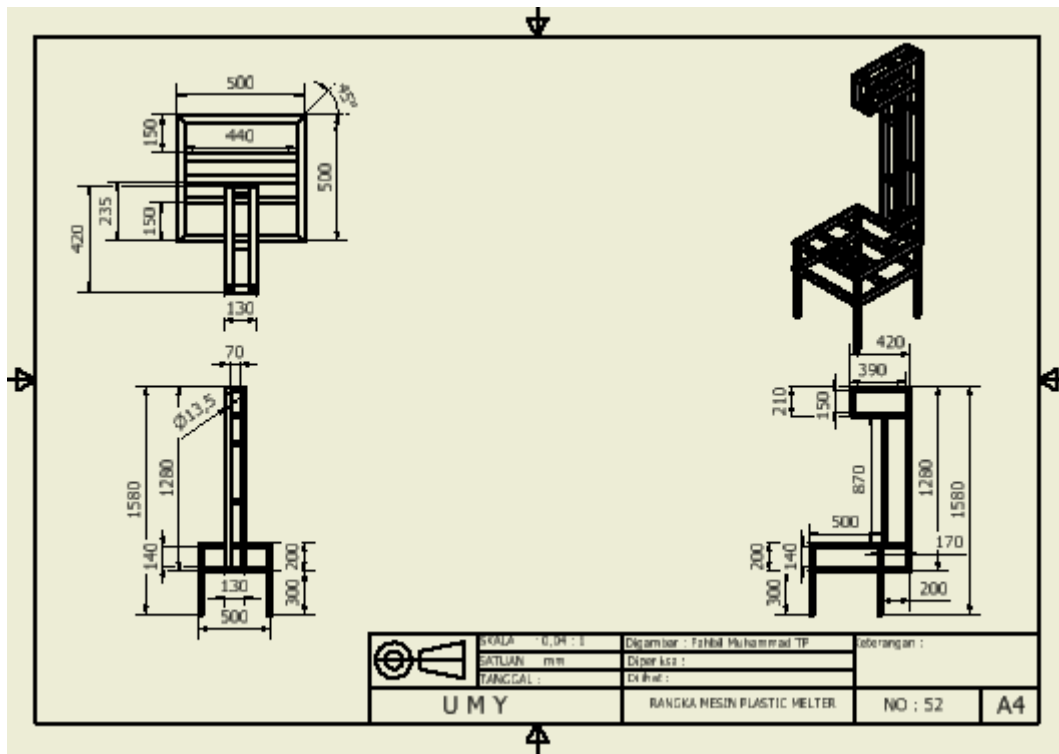
Gambar frame mesin plastic melter
