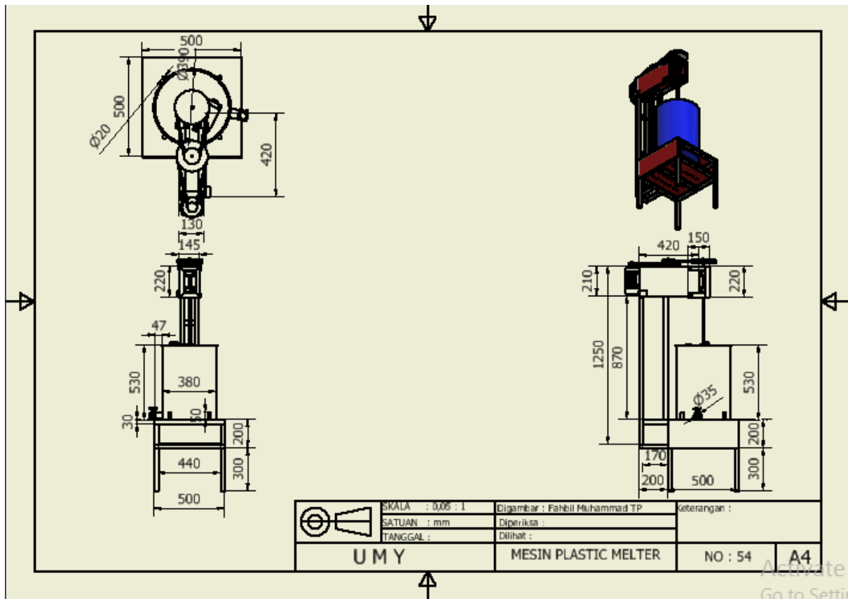
Gambar mesin plastic melter
