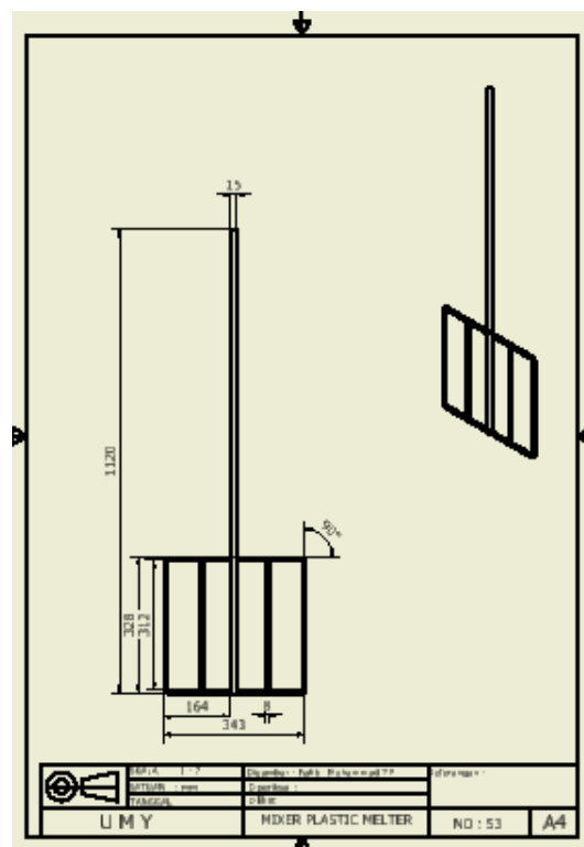
Gambar mixer mesin plastic melter
